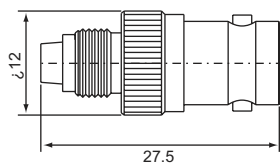
NIPPLE male-F female N1F-312 (50Ω)
