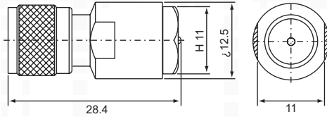
NIPPLE female-mini UHF female NIM-322 (50Ω)
