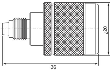
NIPPLE male-SMA female NIS-312 (50Ω)
