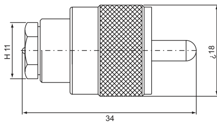
rotating NIPPLE-UHF male NIU-311 (50Ω)
