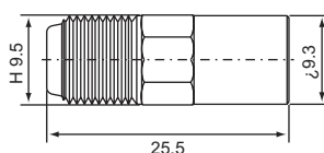
NIPPLE male-F female N1F-312 (50Ω)
