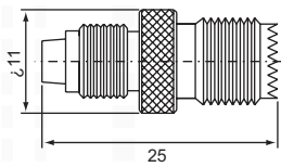
rotating NIPPLE male-N male (50Ω) NIN-311
