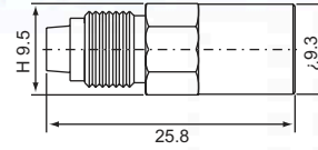
NIPPLE male bulkhead receptacle N1-331 (50Ω)
