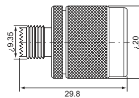
N female-TNC female NT-322 (50Ω,75Ω)
