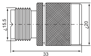
four N female, cross type N-822 (50Ω,75Ω)
