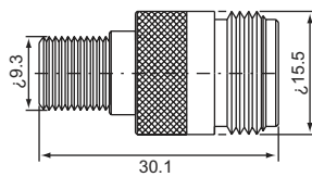
N male-TNC female NT-312 (50Ω,75Ω)
