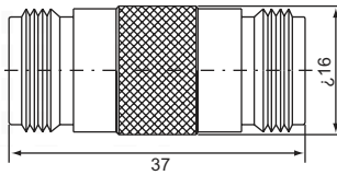
Double N female N-322 (50Ω,75Ω)
