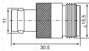
N female-F female NF-322 (50Ω,75Ω)
