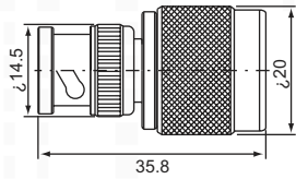
N female-BNC female NB-322 (50Ω,75Ω)
