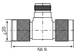
Double N male-single N female T-type N-521 (50Ω,75Ω)
