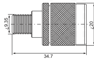
N male-mini UHF female NM-312 (50Ω,75Ω)
