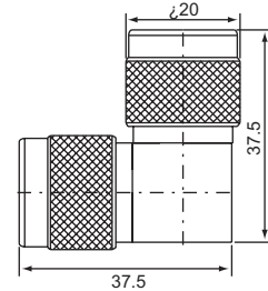
Double N female Right angle N-422 (50Ω,75Ω)
