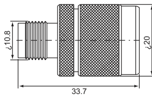
N male-UHF female NU-312 (50Ω,75Ω)
