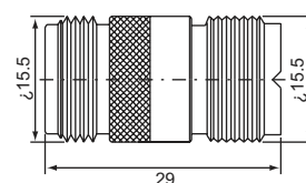
N female-UHF female NU-322 (50Ω,75Ω)
