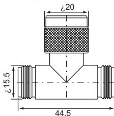
Double N male-single N female T-type N-521 (50Ω,75Ω)
