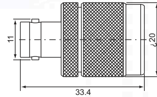
N male-F female NF-312 (50Ω,75Ω)
