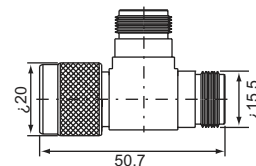
Three N female T-type N-522 (50Ω,75Ω)
