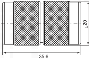
Double N female N-322 (50Ω,75Ω)
