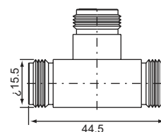
Three N female T-type N-522 (50Ω,75Ω)
