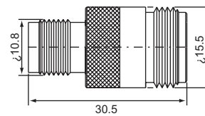
N female-UHF female NU-322 (50Ω,75Ω)
