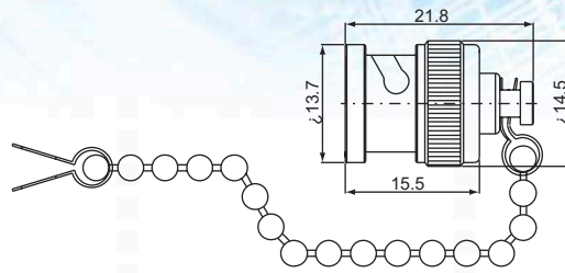
BNC MALE, Protective cap B-61P
