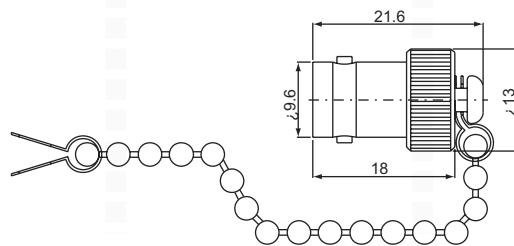
BNC FEMALE, Protective cap B-62P
