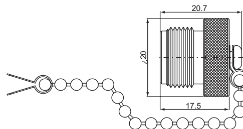
N FEMALE, Protective cap N-62P
