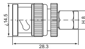
SMA male-BNC male SB-311 (50Ω)
