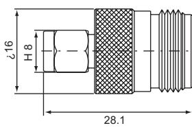
SMA female-N female SN-322 (50Ω)
