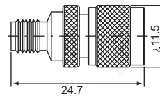
SMA male-N male SN-311 (50Ω)
