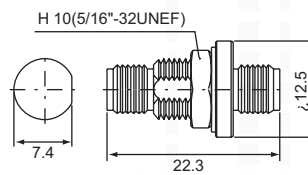
SMA male-SMA female right angle S-412 (50Ω)
