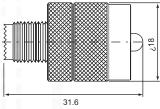
UHF male-RCA female (50Ω,75Ω) UR-312
