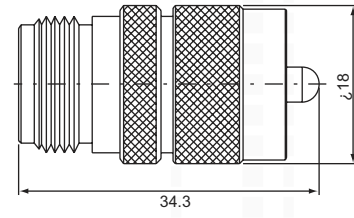
UHF male-TNC female (50Ω,75Ω) UT-312
