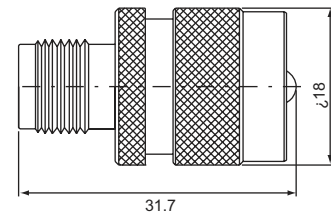
UHF male-TNC female (50Ω,75Ω) UT-312
