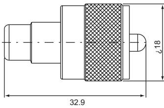
UHF male-RCA female (50Ω,75Ω) UR-312
