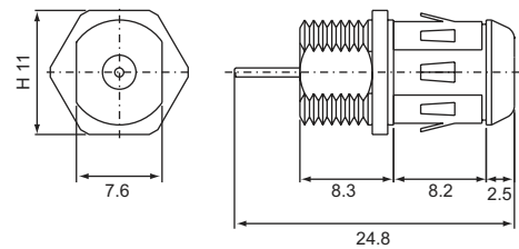
GSK FEMALE, Solder type G-P215 PCB mount
