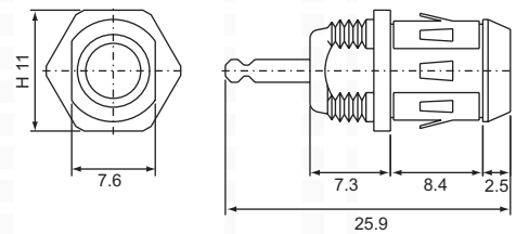
GSK FEMALE, Solder type G-235-2 Bulkhead receptacle
