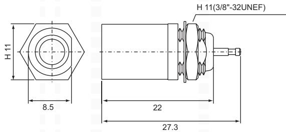
GSK MALE, Solder type G-235-1 Bulkhead receptacle
