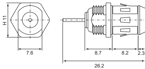
GSK MALE, Solder type G-235-3 Bulkhead receptacle
