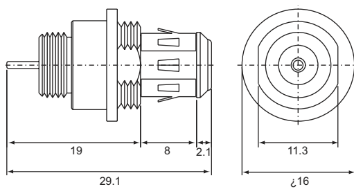
GSK female-F female GF-322-D (75Ω)
